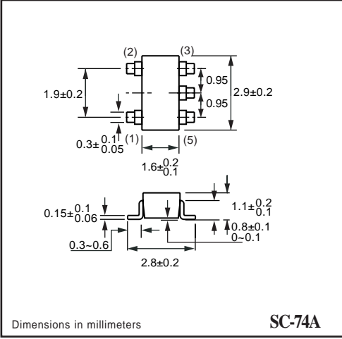
SC-74A
